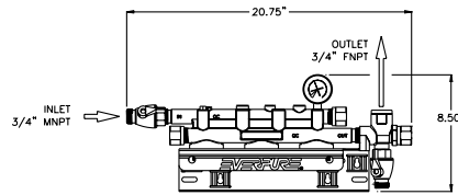
QC71 Triple Head: EV9272-23
