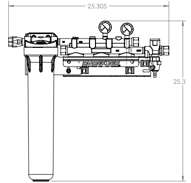
Coldrink/Insurice Triple Manifold with 20" Prefilter: EV9293-23
