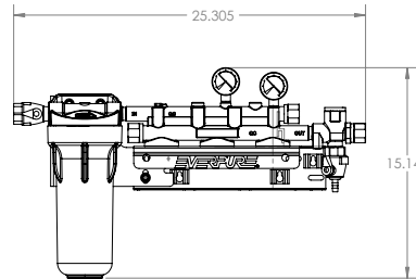
Coldrink/Insurice Triple Manifold with 10" Prefilter: EV9293-03
