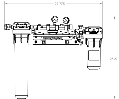
High Flow Triple Manifold with CSR 20" Prefilter: EV9294-23
