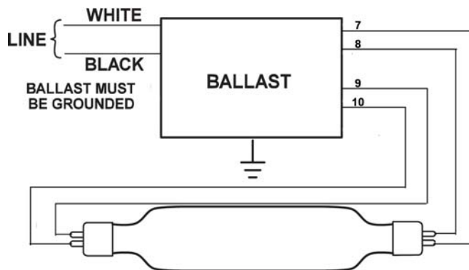
Wiring Diagram 1
