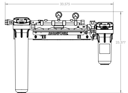
High Flow CSR Quad Manifold with 20" Prefilter: EV9294-24
