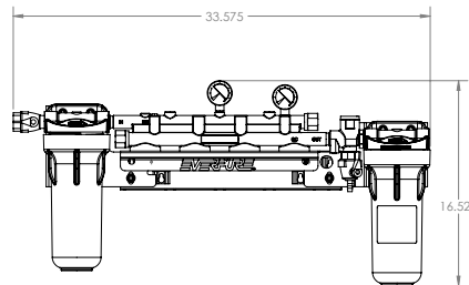
High Flow CSR Quad Manifold with 10" Prefilter: EV9294-04
