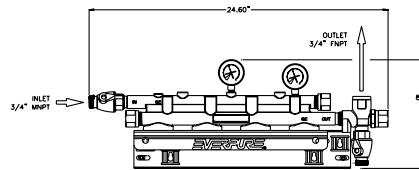
QC71 Quad Head: EV9336-11
