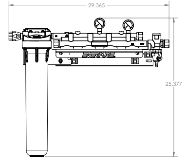
Coldrink/Insurice Quad Manifold with 20" Prefilter: EV9293-24
