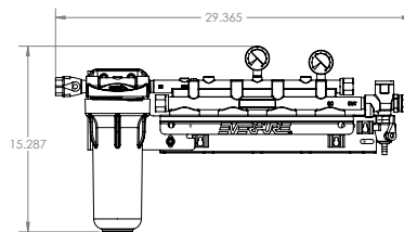
Coldrink/Insurice Quad Manifold with 10" Prefilter: EV9293-04
