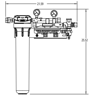
Coldrink/Insurice Twin Manifold with 20" Prefilter: EV9293-22
