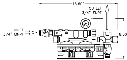
QC71 Twin Head: EV9272-22
