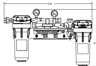
High Flow CSR Twin Manifold with 10" Prefilter: EV9294-02
