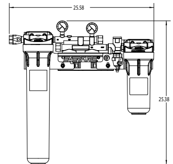
High Flow CSR Twin Manifold with 20" Prefilter: EV9294-22
