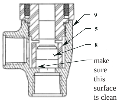
B-0968/B-0969 Cross-section
