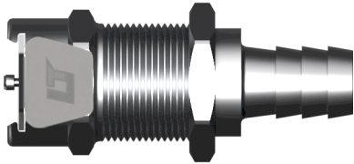
40CBV-SB3-06N3 LinkTech 40CB Series Panel Mt. Socket, Valved, 3/8" HB Chrome Brass, NSF 61 Buna N
