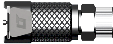
40CBV-SB9-06N3 LinkTech 40CB Series Inline Socket, Valved, 3/8" PTF NSF 51 Acetal, NSF 61 Buna N
