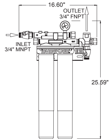
QC7I Twin 7CLM EV9278-12
