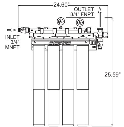
QC7I Quad 7CLM EV9278-14
