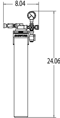
QC7I Single 7CLM EV9278-11
