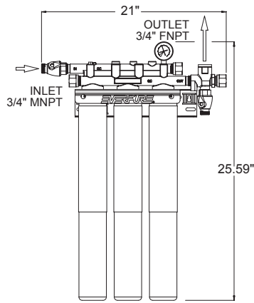
QC7I Triple 7CLM EV9278-13
