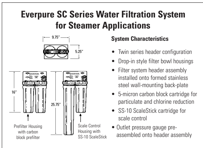
Figure 3 - Dimensions
