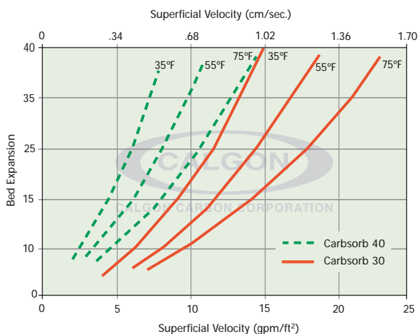
Typical Bed Expansion Backwashed and Segregated Bed
