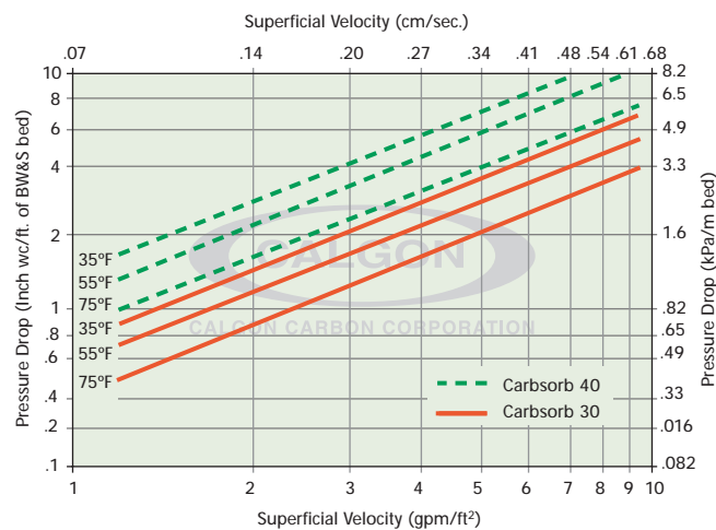
Typical Downflow Pressure Drop Curve Backwashed and Segregated Bed
