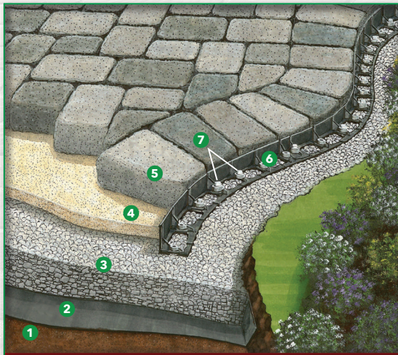
Strong Interlocking Joint with Built-In Spike-Through Connector
