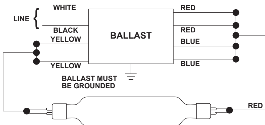
Wiring Diagram 1
