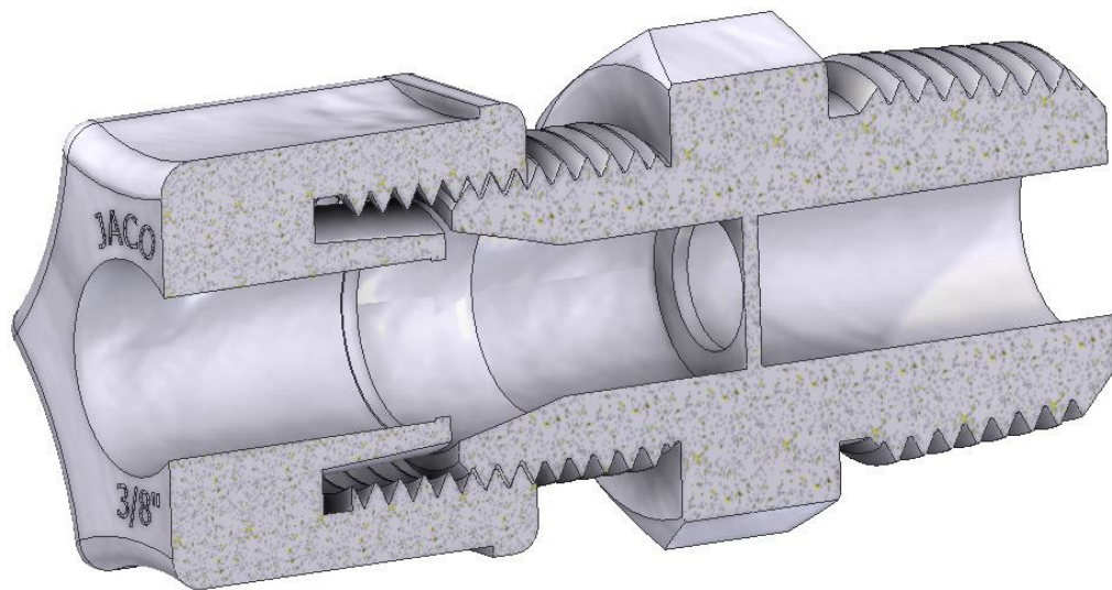
Fig.1 – View shown with Standard Ferrule Nut (O – Nut)
