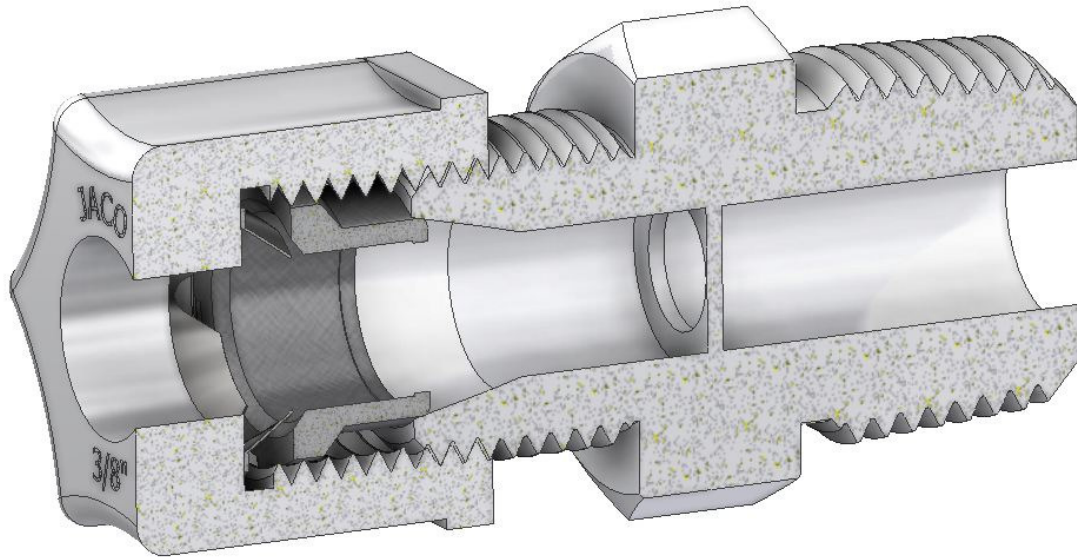
Fig.3 – View shown with Stainless Steel Gripper Nut (SG – Nut)
