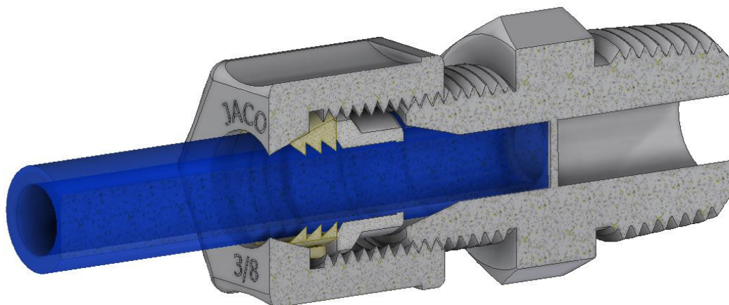
Fig.4 – View shown with Plastic Gripper Nut (PG – Nut) & Plastic Tubing
