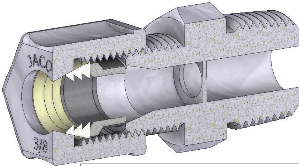
Fig.2 – View shown with Plastic Gripper Nut (PG – Nut)
